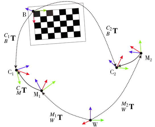
Fig. 4: Intrinsic and extrinsic calibration scene. Camera frame from C_1 to C_2 , and the markers which attached with the camera rigidly move from M_1 to M_2 correspondingly. W is the world frame of MoCap system and frame B is fixed on the checkerboard pattern. During the calibration, we keep the checkerboard motionless.
